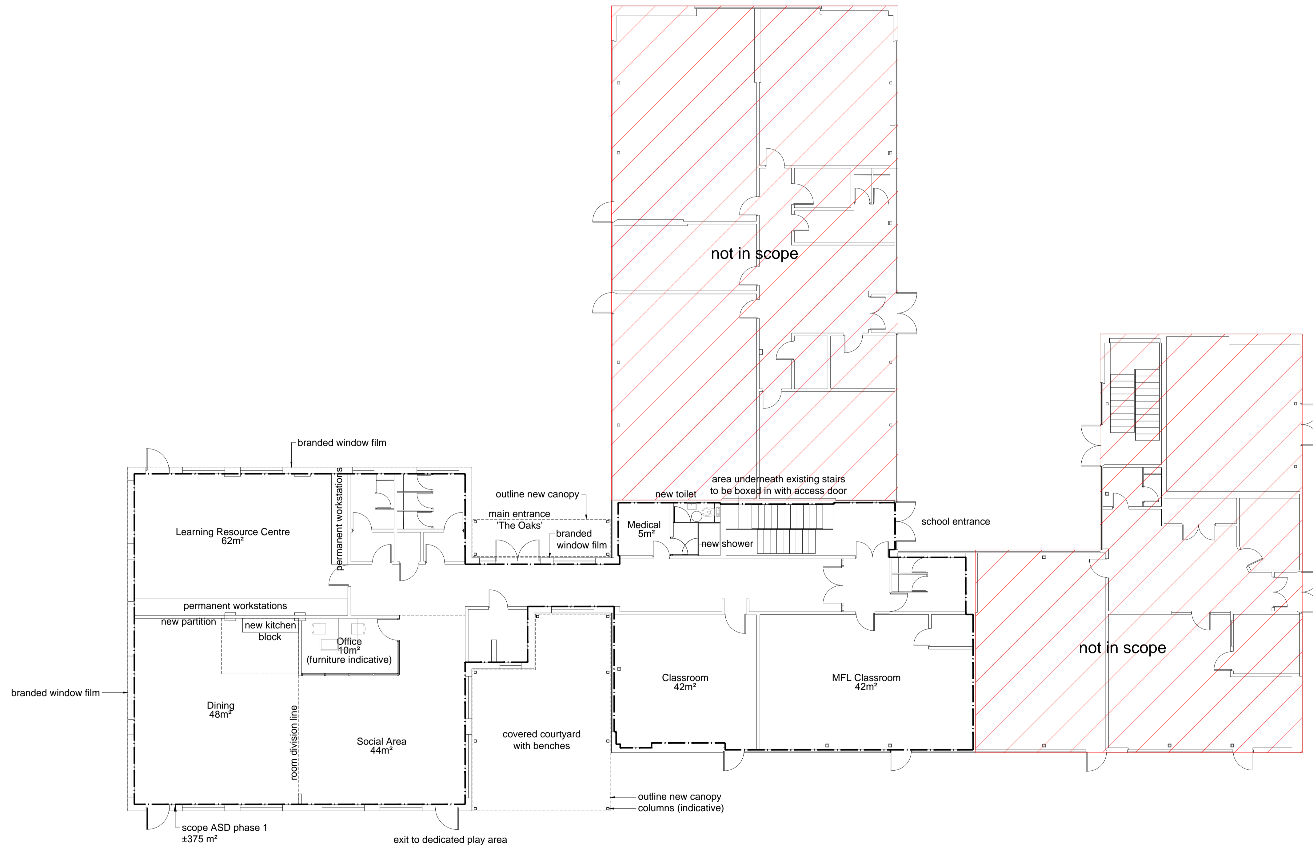
PROPOSED GROUND FLOOR (ASD PHASE 1)
