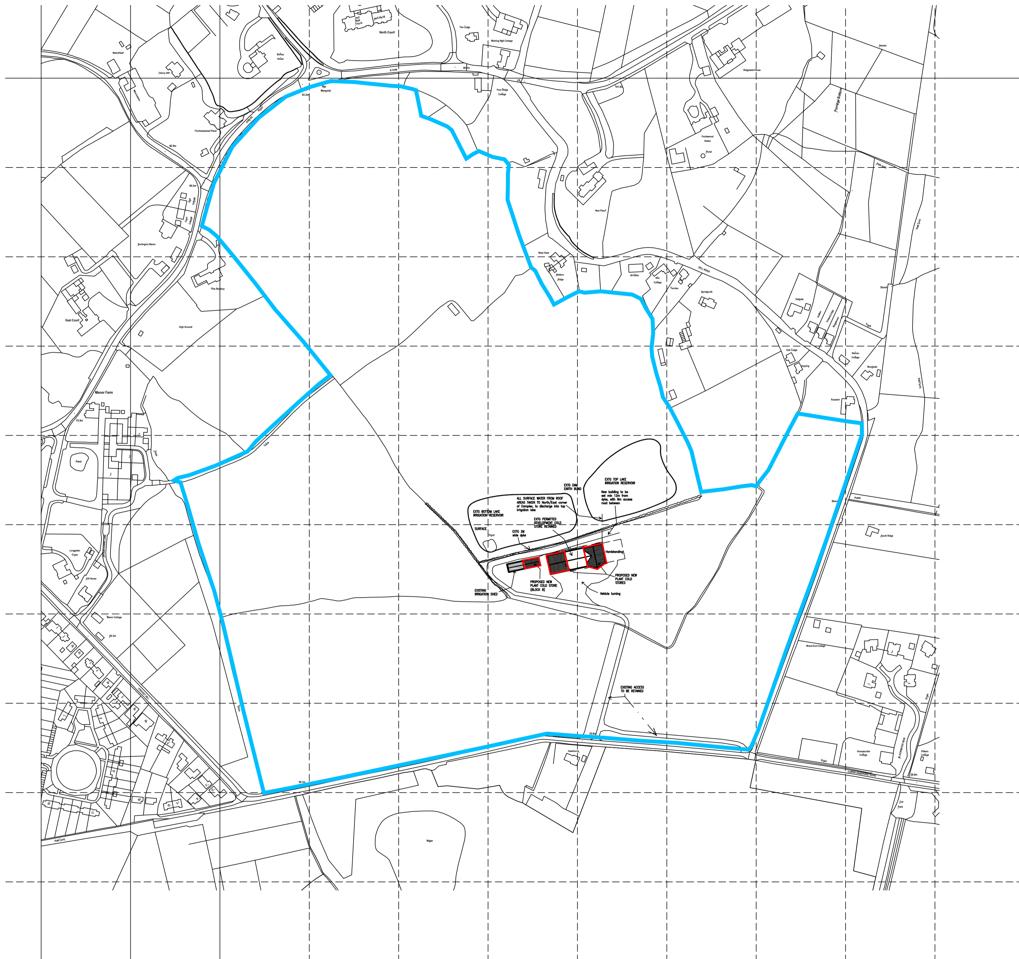
LOCATION PLAN 1:2500
