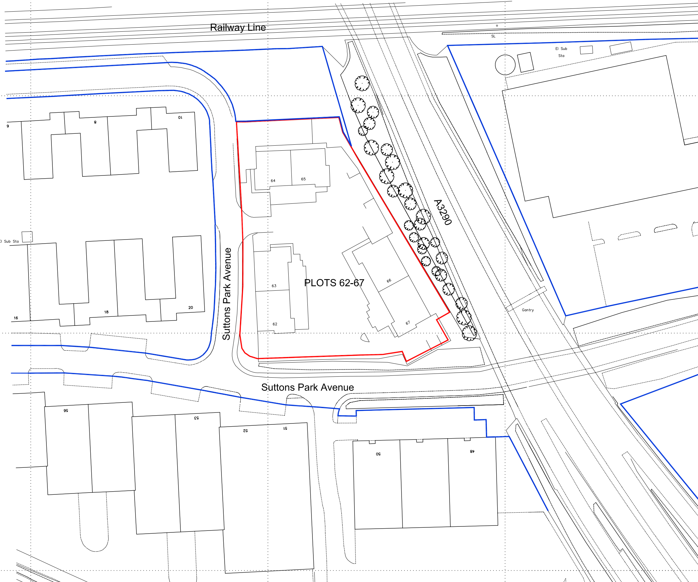
01 LOCATION PLAN 100 1:500 113
