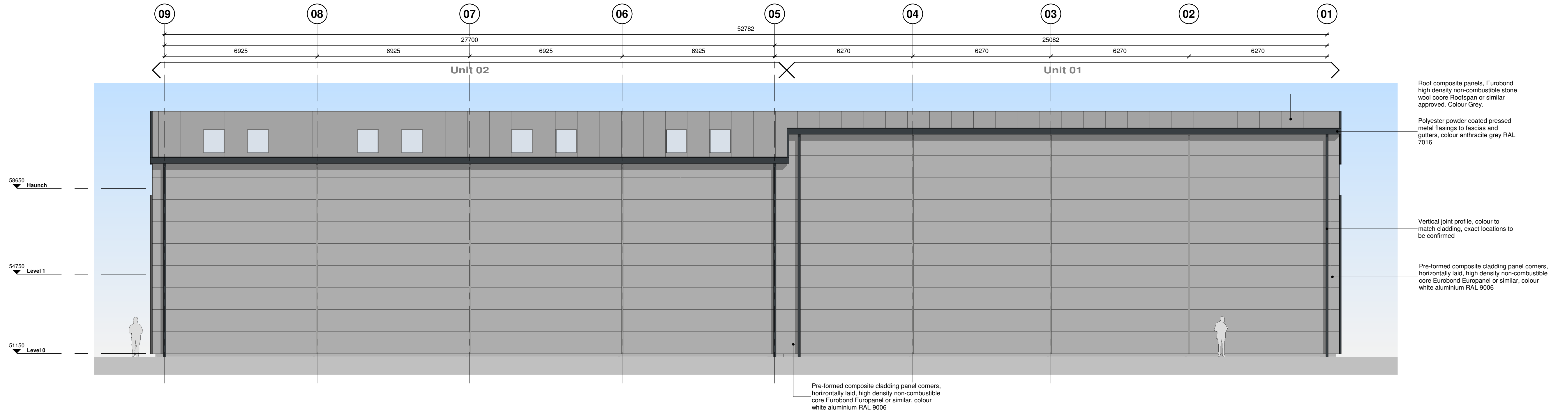
C Elevation C (North-West, Rear) 1 : 100
