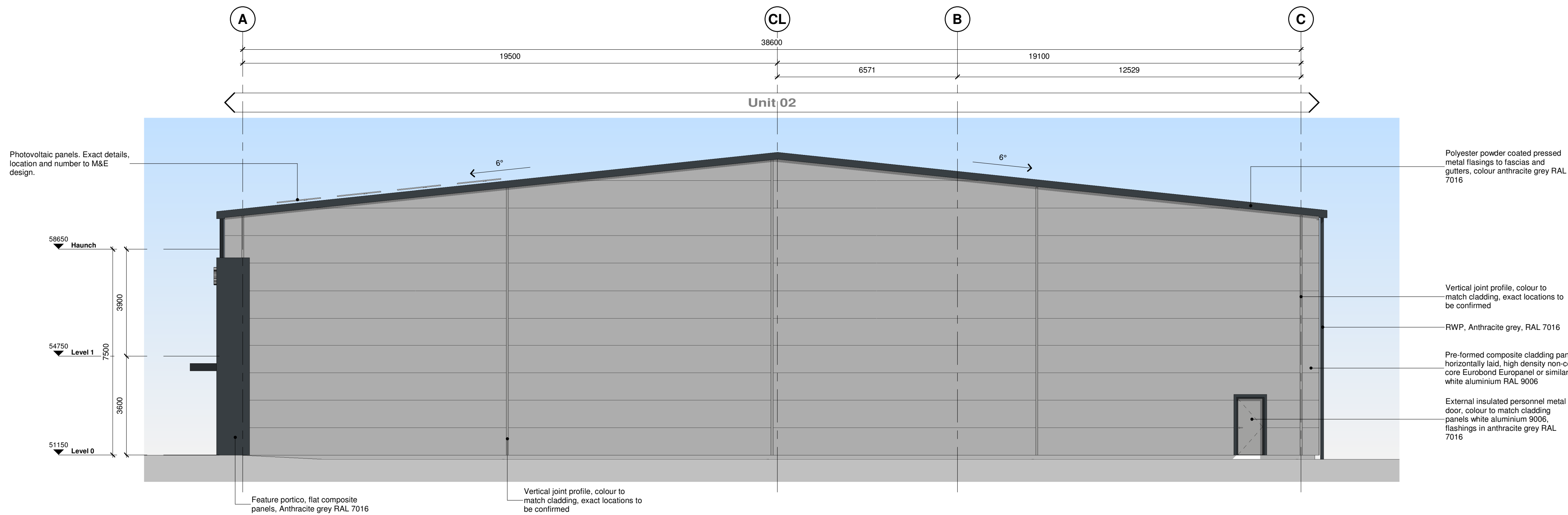
D Elevation D (North-East, Side path) 1 : 100
