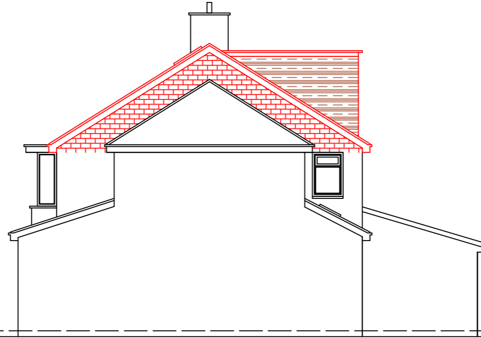
PROPOSED SIDE-1 ELEVATION
