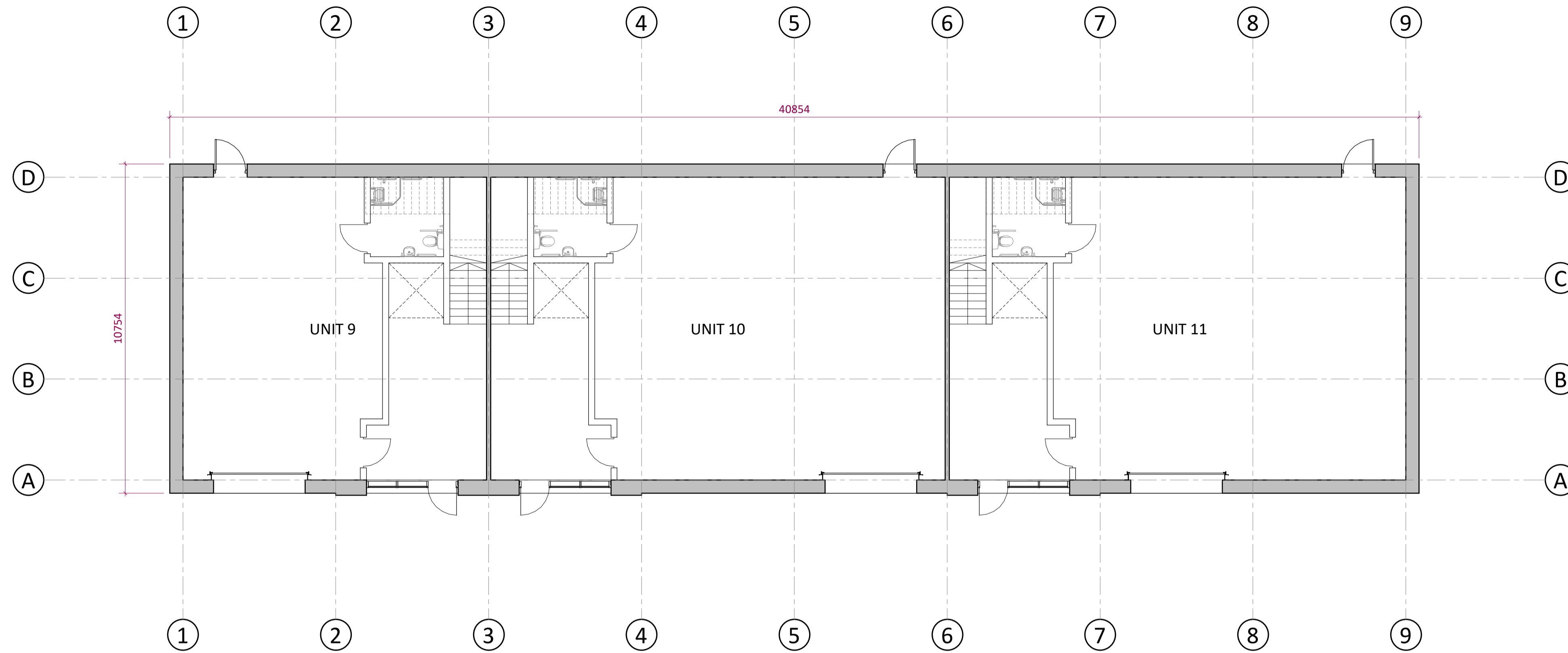
GROUND FLOOR 1 : 100
