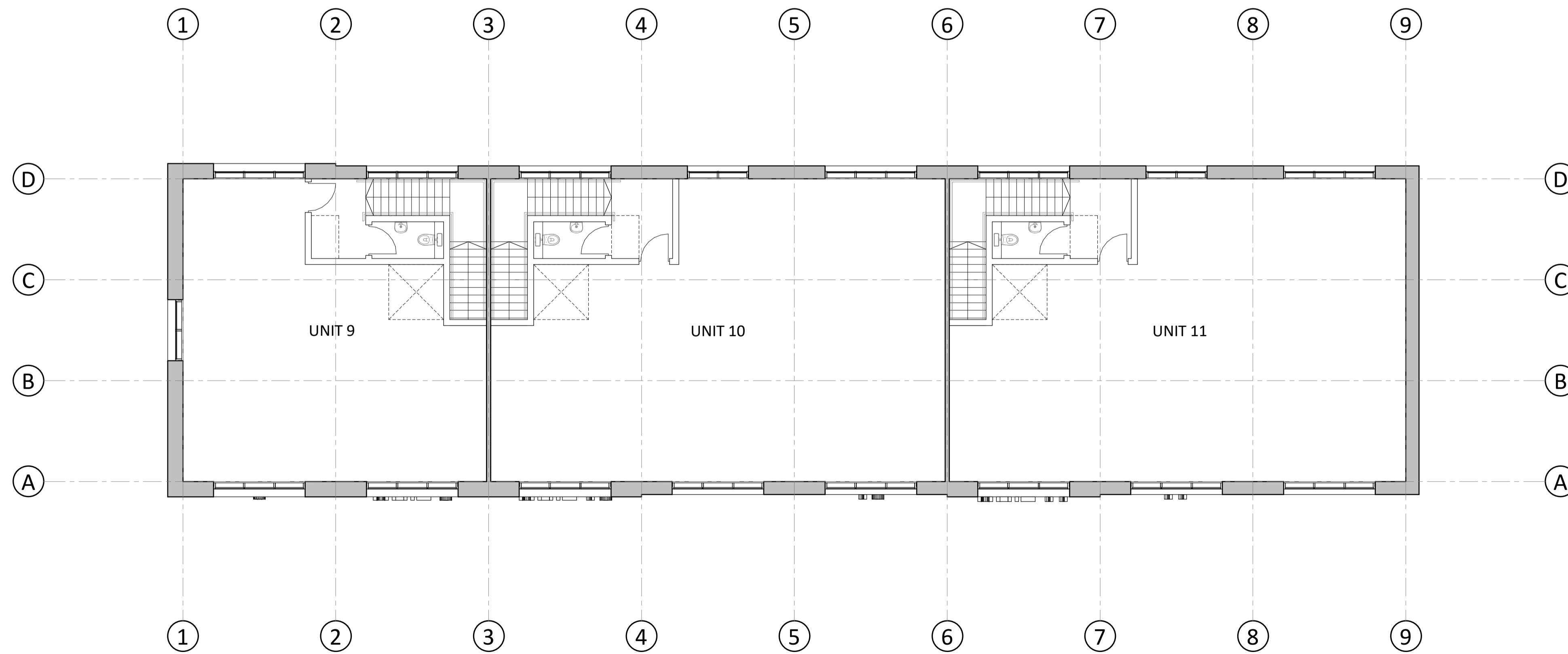
FIRST FLOOR 1 : 100
