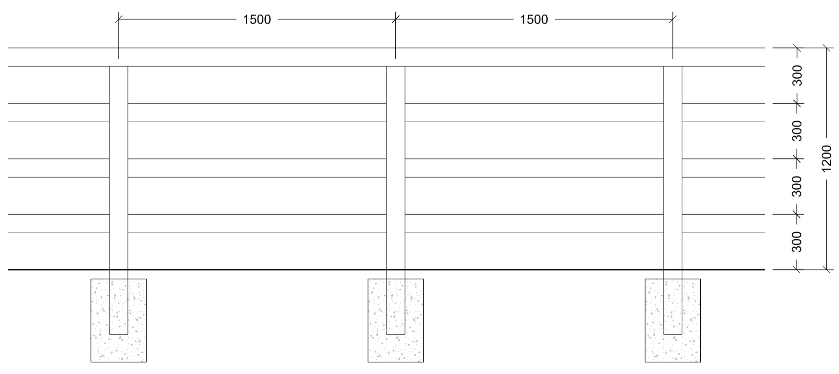
PROPOSED TIMBER FENCE DETAIL 1:20
