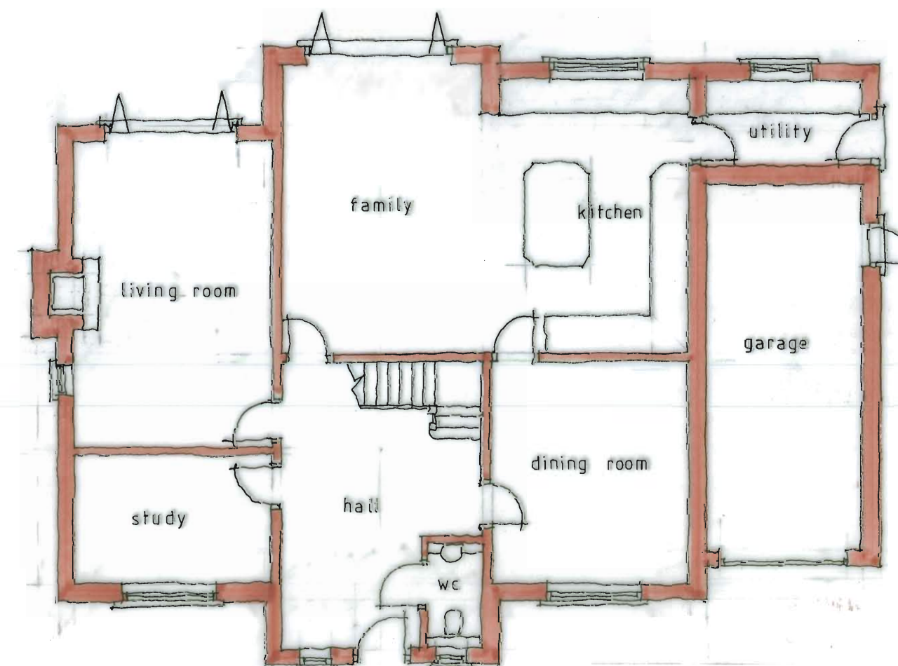
GROUND FLOOR
