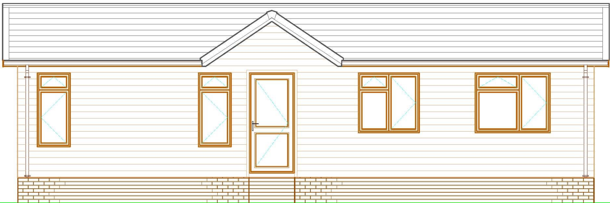
Nearside Elevation
