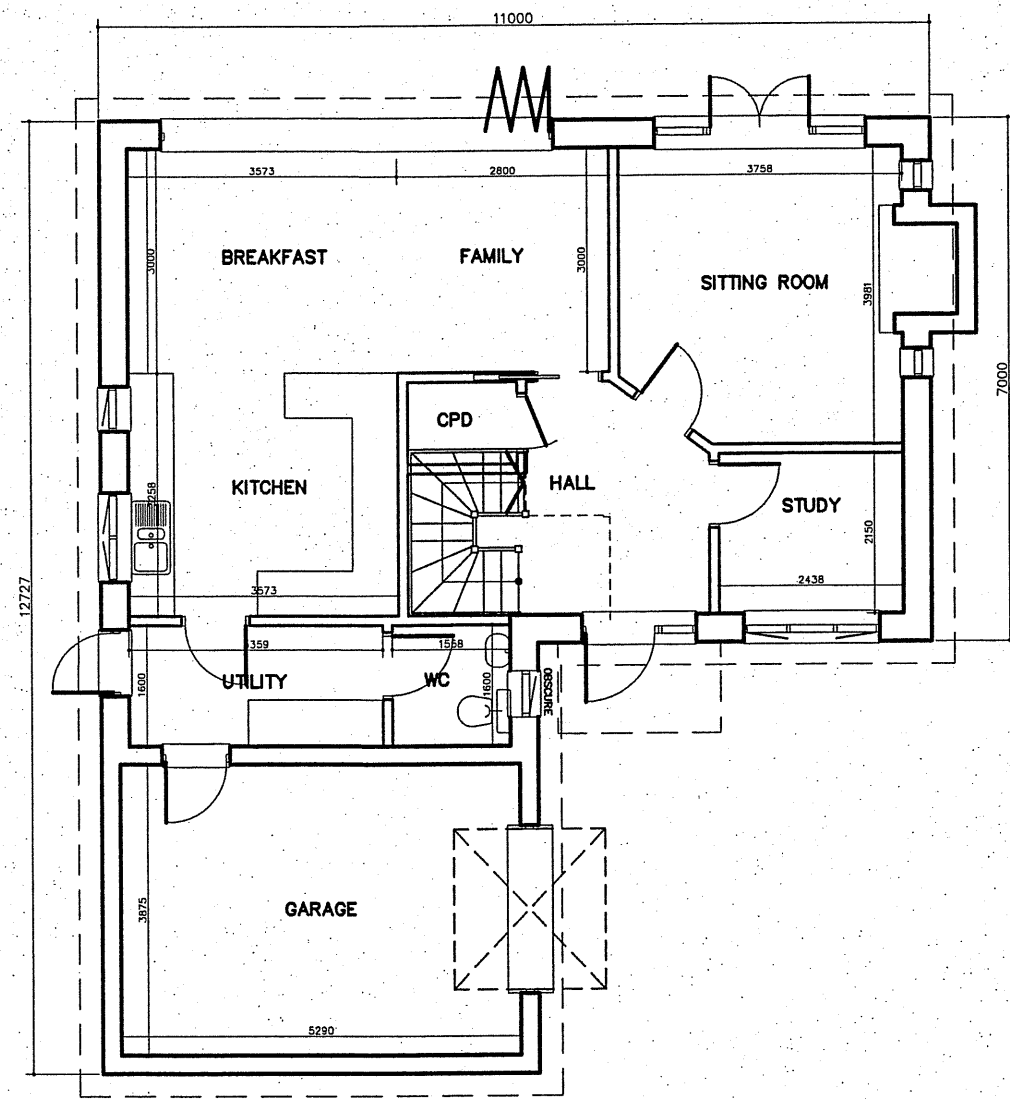
GROUND FLOOR EXTERNAL AREA 106.88 sq.m
